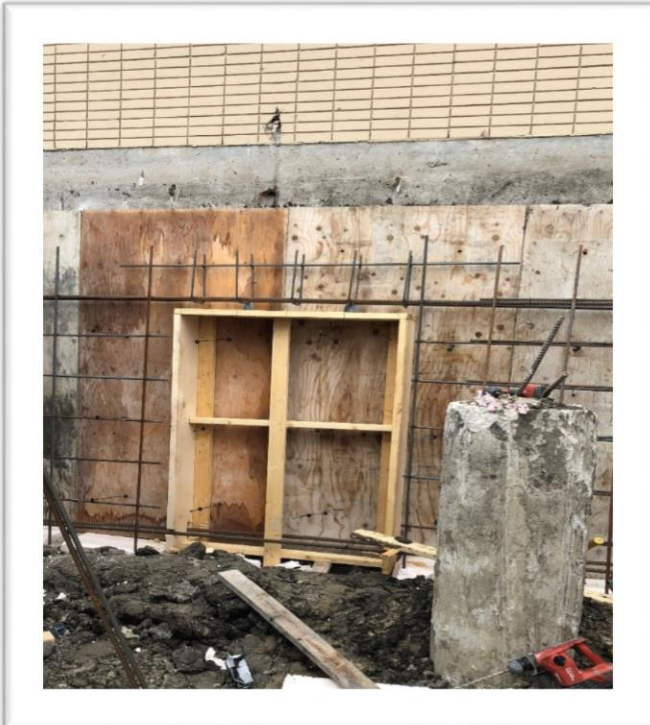
Completed Utilidor
