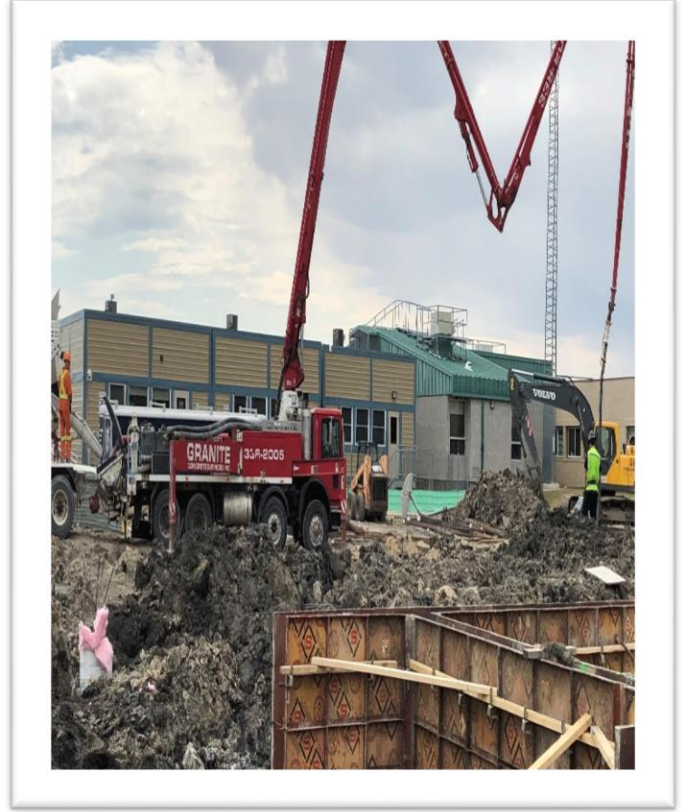
Concrete pump Truck pouring concrete
