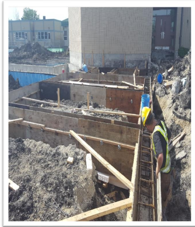
Framing footing walls North side
