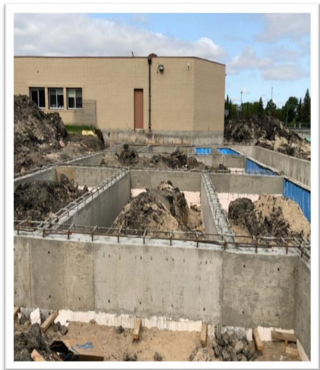
Footings for 3 classrooms completed
